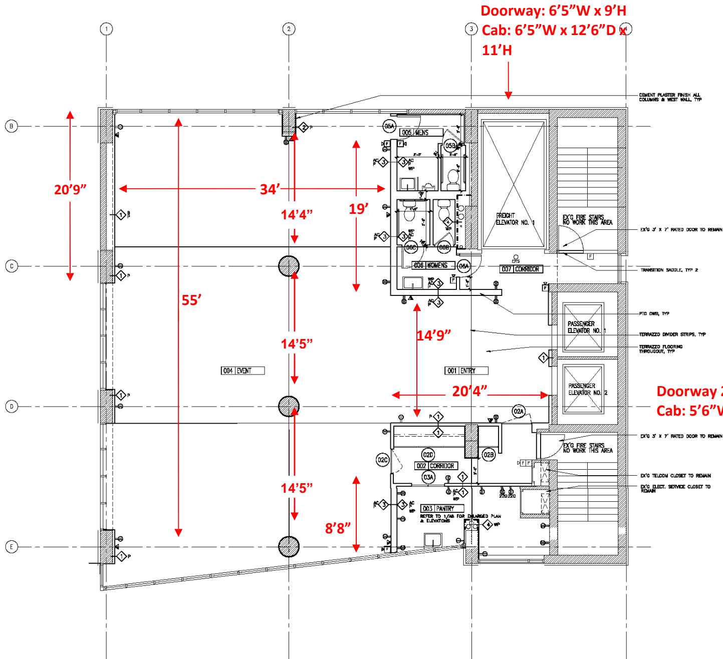
1 FLOOR PLAN 1/4"=1'-0"
